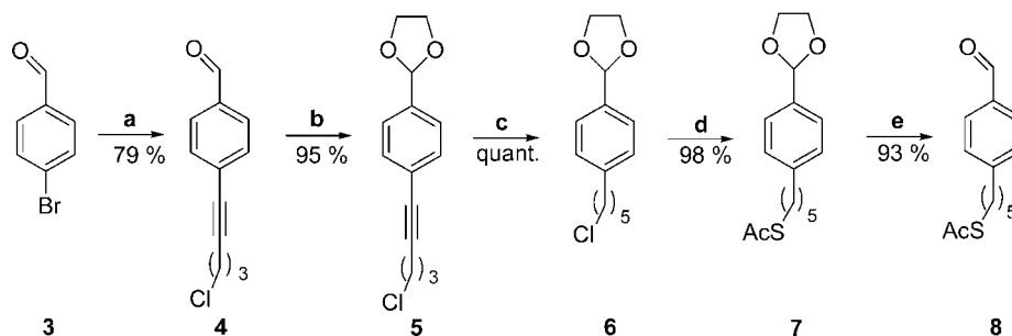
Scheme 2. Reagents and conditions: a . 5-chloro-1-pentyne, Pd(OAc) 2 , PPh 3 , NEt 3 , CuI, THF, room temp. overnight; b . ethylene glycol, TsOH, benzene, reflux, 12 h; c . RhCl(PPh 3 ) 3 , H 2 , benzene, room temp. 14 h; d . KSac, reflux, 13 h, 56 °C; e . TsOH, acetone, H 2 O, reflux, 14 h.
