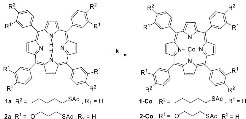
Scheme 5. Reagents and conditions: k, Co(OAc) 2 ·4H 2 O, DCM/MeOH, 4:1, reflux, 2 h.
