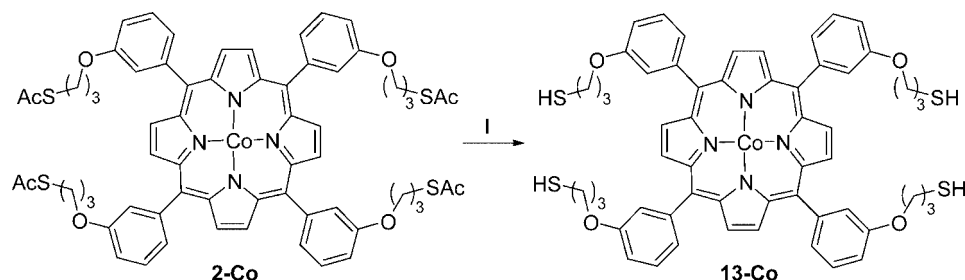
Scheme 6. Reagents and conditions: I. \text{HCl}_{(\text{aq.})} , DMF, room temp.
