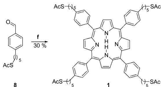
Scheme 3. Reagents and conditions: 1: pyrrole, TFA, DCM, room temp., 1.5 h, 2: p -chloranil, reflux, 1 h.
