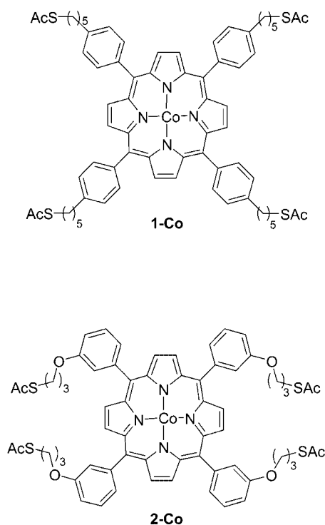
Figure 1. Thioacetate-functionalized cobalt(II) porphyrins for immobilization on gold surface.
