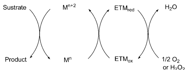
Scheme 1. Biomimetic oxidation involving electron-transfer mediator (ETM).
