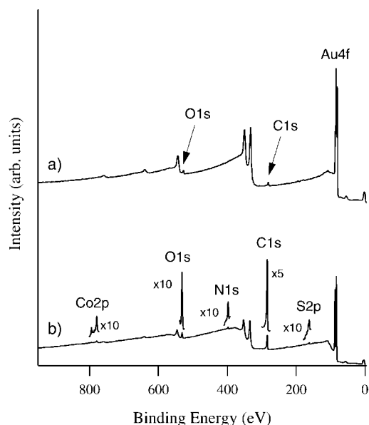
Figure 2. a) Photoelectron spectrum obtained at a take off angle (TOA) of 10^\circ of the bare Au surface prior to molecular deposition. The peaks corresponding to carbon and oxygen contamination are marked. All other features in the spectrum are related to the Au substrate. The most intensive photoemission line for Au is also marked (Au4f). b) Photoelectron spectrum at a TOA of 10^\circ of 13-Co (deprotected 2-Co ) on the Au surface. The different atomic constituents of the molecule are present and marked in the spectrum.
