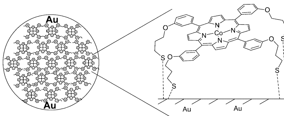
Figure 3. Immobilization of cobalt porphyrin on a gold surface via sulfur tails.
